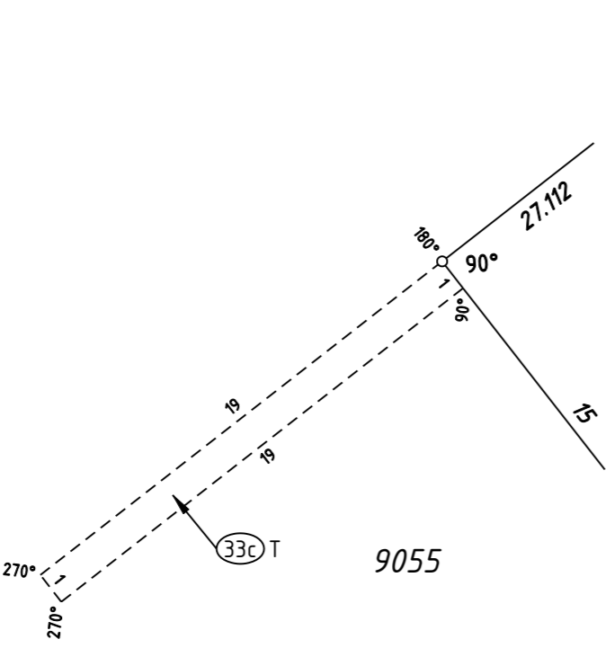
ENLARGEMENT 'I2' NOT TO SCALE
