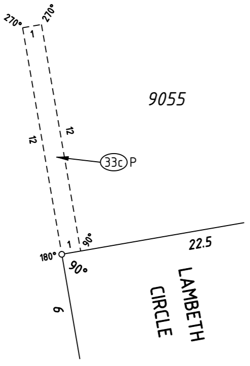
ENLARGEMENT 'E2' SCALE 1:200
