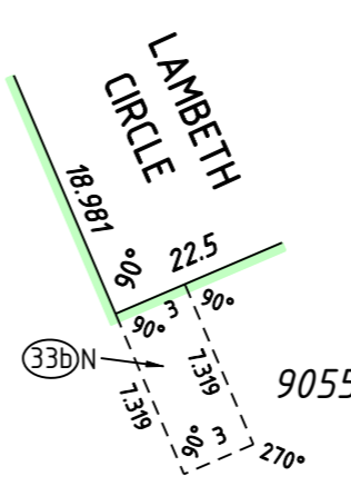
ENLARGEMENT 'T' NOT TO SCALE
