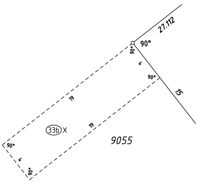
ENLARGEMENT 'I1' NOT TO SCALE
