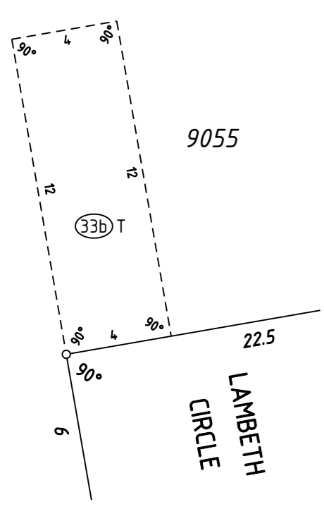
ENLARGEMENT 'E1' SCALE 1:200
